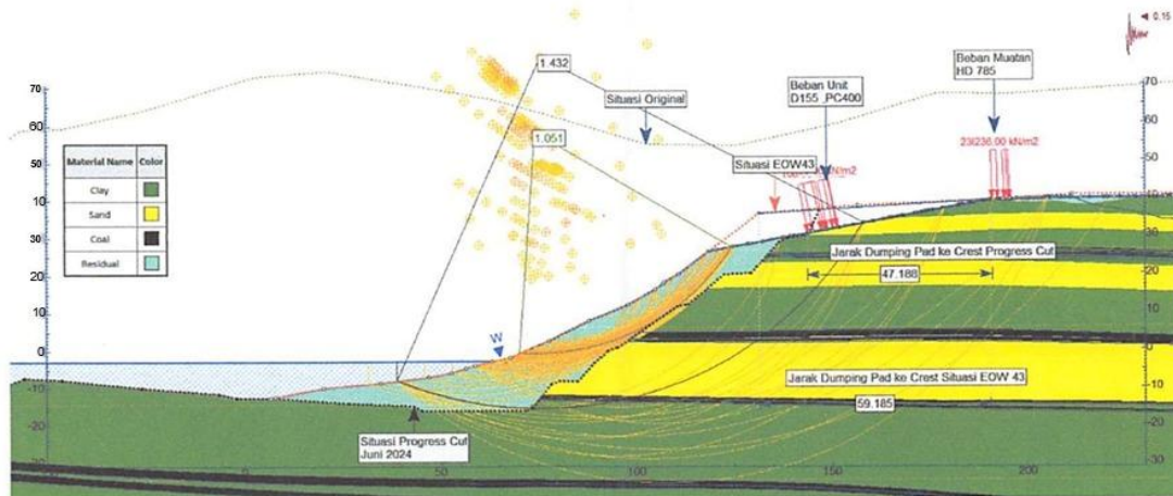
Figure 2. The result of geotechnical analysis
